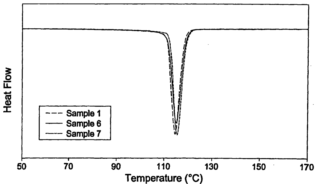
Fig. 6 DSC Crystallization of Plasticized Metallocene Propylene Polymers
